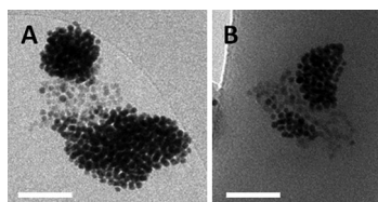
Figure 5. A) and B) Representative cryo-TEM images of segregated assemblies formed upon treating 2-capped \gamma -Fe 2 O 3 NPs with TOAB-capped AuNPs. Scale bar = 50 nm.
